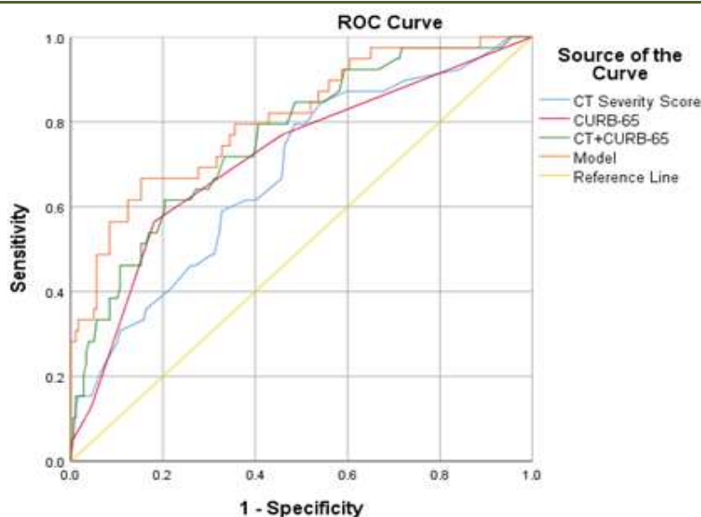
Figure 1: ROC curves for CTSS and CURB-65 scoring system to predict in-hospital mortality
